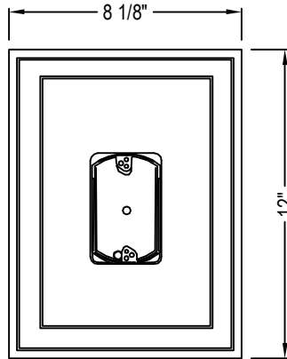
JUMBO ELECTRICAL BLOCK - CENTERED
