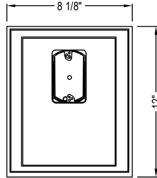
JUMBO ELECTRICAL BLOCK - OFFSET
