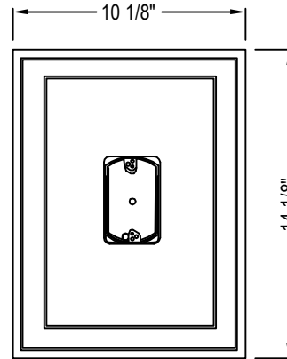
SUPER JUMBO ELECTRICAL BLOCK - CENTERED
